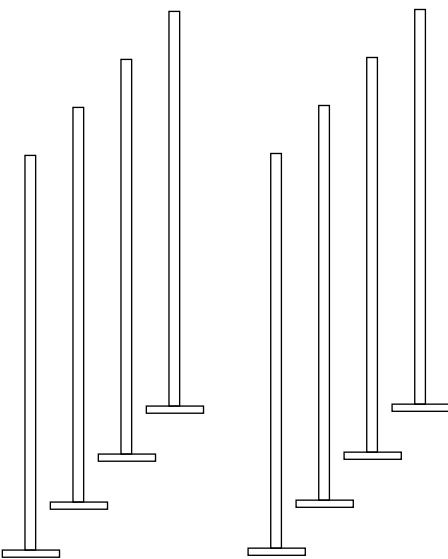
Vertical Poles w/Flange (8) 74.0" x 2.0"OD
